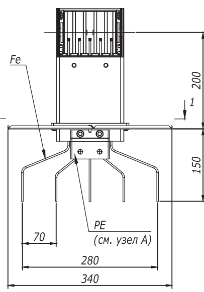
3P+N+PE+FE
