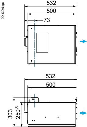
KSB400DB12
