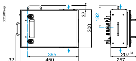
KSB160SG4
