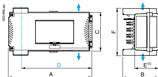
KSB63SM ●8, KSB100SM ●12
