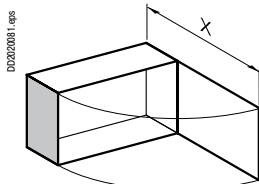
X = 577.5 (KSB160SE●) X = 777 (KSB250SE●) X = 855 (KSB400SE●)
