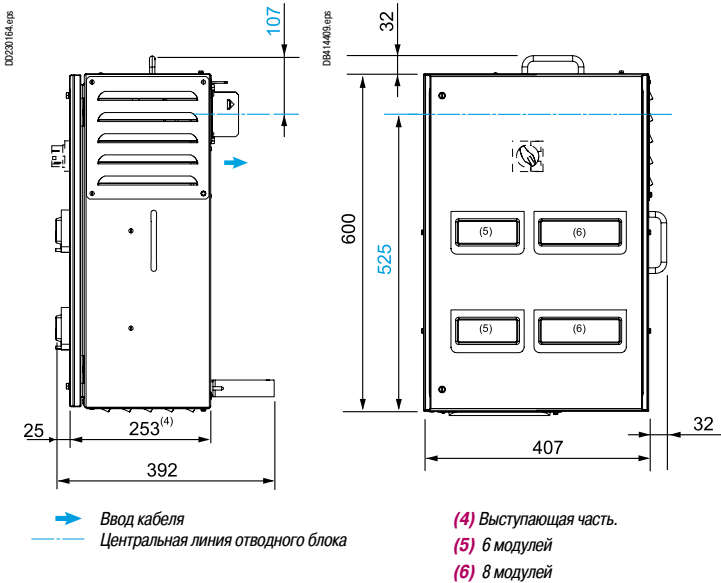
KSB250SM428
