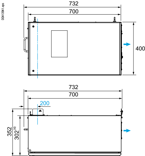
KSB400DB12
