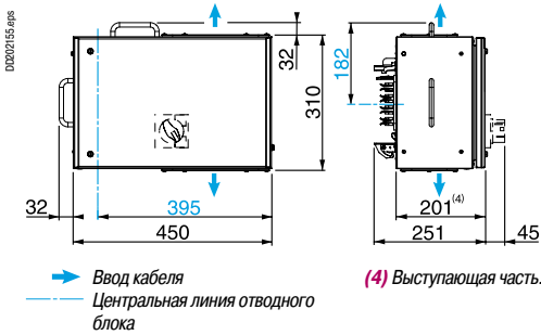
KSB160SM13
