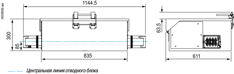
KSB630SE●
