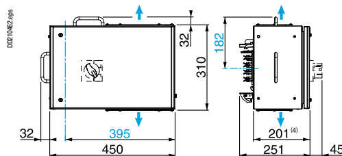
KSB160DC●
