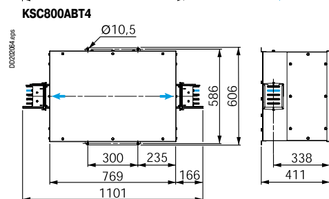
KSC800ABT4
