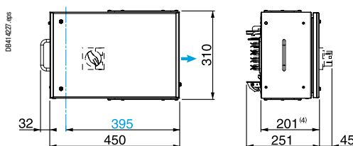
KSB250SDF4
