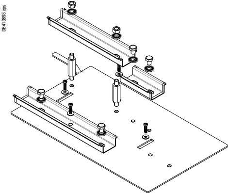
KSB63PMP
