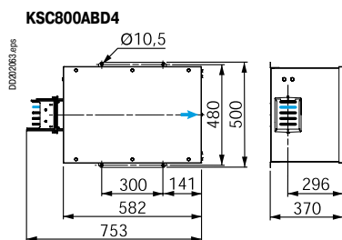
KSC800ABD4
