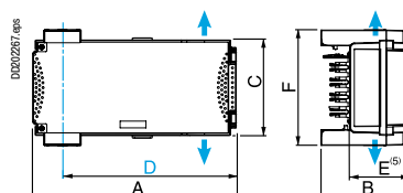
KSB32SG4, KSB80SG4
