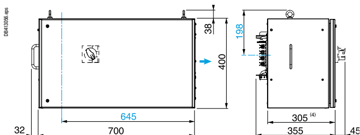
KSB400SDF4
