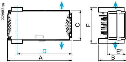
KSB50SF●, KSB100SF●
