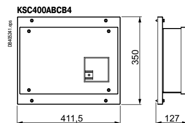
KSC400ABCB4
