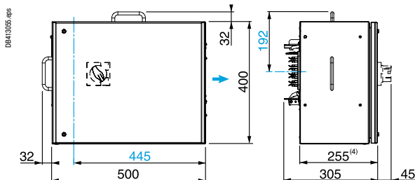
KSB250SDF4
