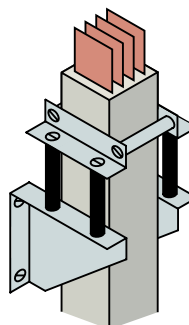
LR..-BF
