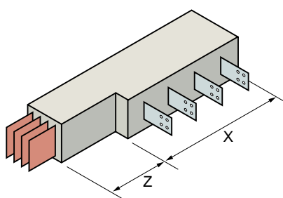
LRC...-TC
