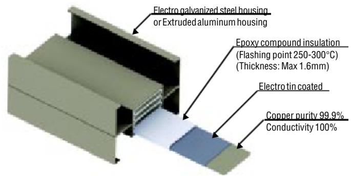
Copper Busduct System
