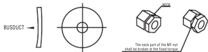
BELLEVILLE WASHER
