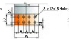
Bar Width: 175-185mm Figure 1.7
