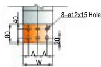
Bar Width: 125-150mm Figure 1.6
