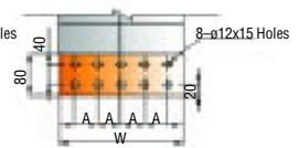
Bar Width: 220-240mm Figure 1.8
