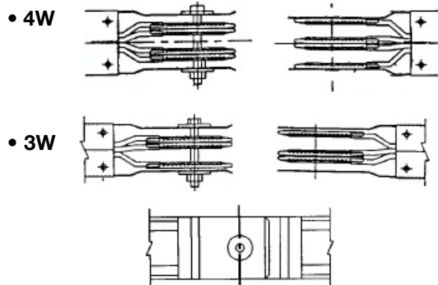
Able to insert from either direction.
