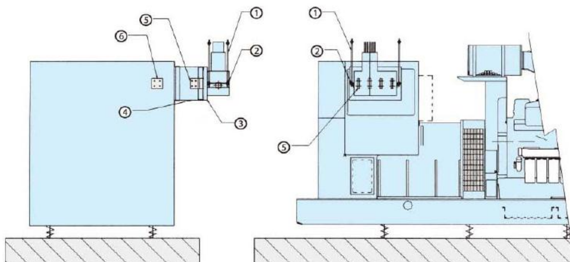
Generator
