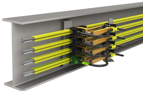
Lateral installation of conductor rails / Horizontal insertion of Current Collectors
