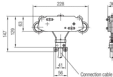
Connection cable
