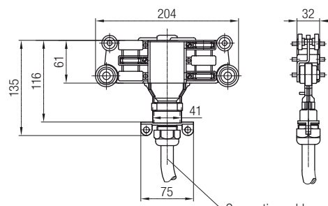
Connection cable
