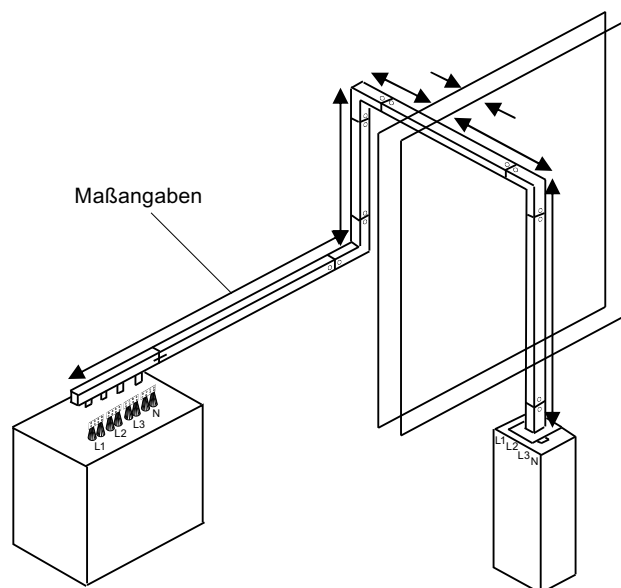
Figure 4-1 Busbar layout with dimension data
